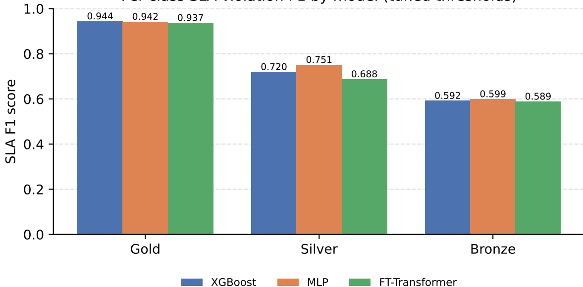
Per-class SLA-violation F1 by model (tuned thresholds)
